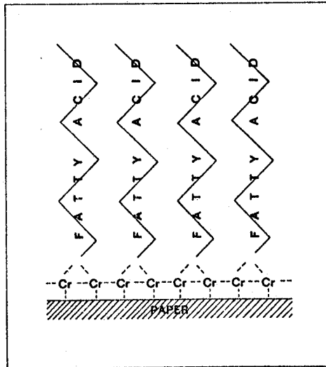
Bonding of "Quilon" Chrome Complex to Paper
